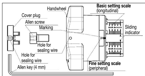
Illustr. 7.1 Presetting
