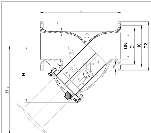
Illust. 2: Dimensions
