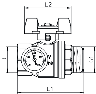
Abb. 5: Dimensions ball valve
