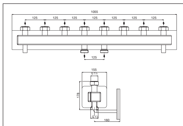
Dimensions distributor DN 25, 4-fold
