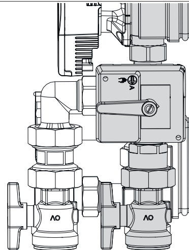
Illust. 23: Switch position of the switching valve (heating mode)
