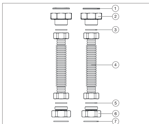
Illust. 36: Construction of the connection set
