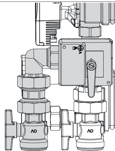
Illust. 24: Switch position of the switching valve (storage cylinder loading)
