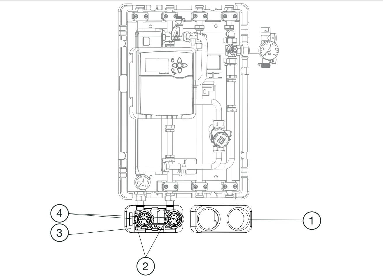
Illust. 7: Transmission station with ball valve connection set
