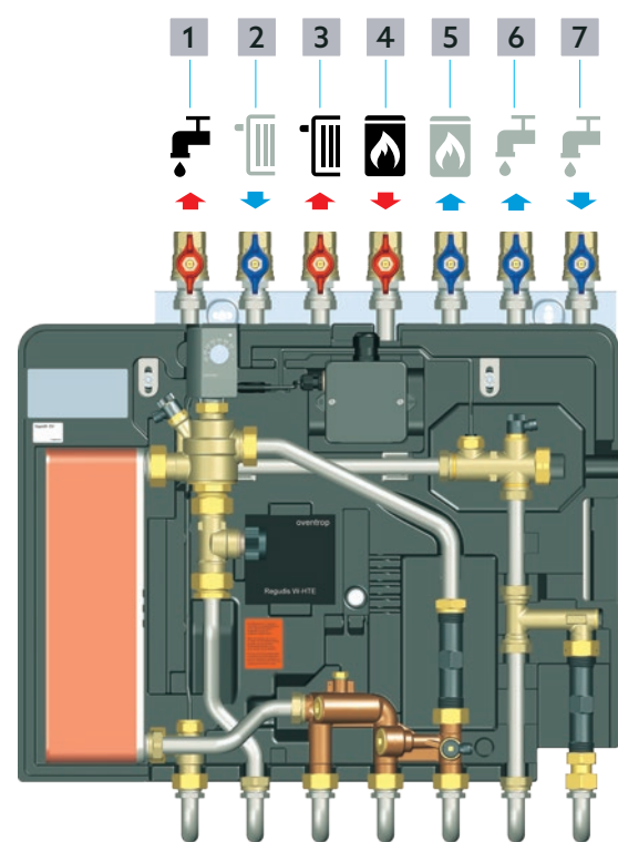
Fig. 5: Connection assignment
