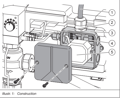
Illustr. 1: Construction
