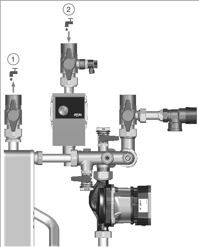
Illust. 10: Functional description (example with high-efficiency pump)
