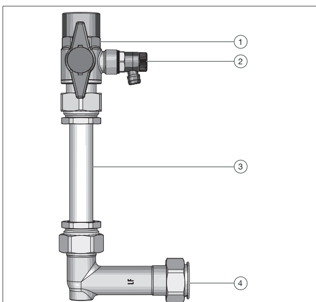
Illust. 2: Construction of the circulation set without high-efficiency pump (item no. 1381152)
