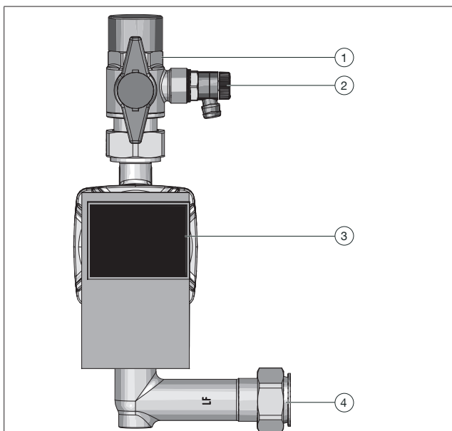
Illust. 1: Construction of the circulation set with high-efficiency pump (item no. 1381150)
