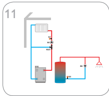
1 mixed heating circuit with central outdoor sensor (slave) and circulation
