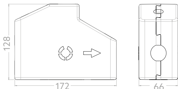
Fig. 5: Insulation shells
