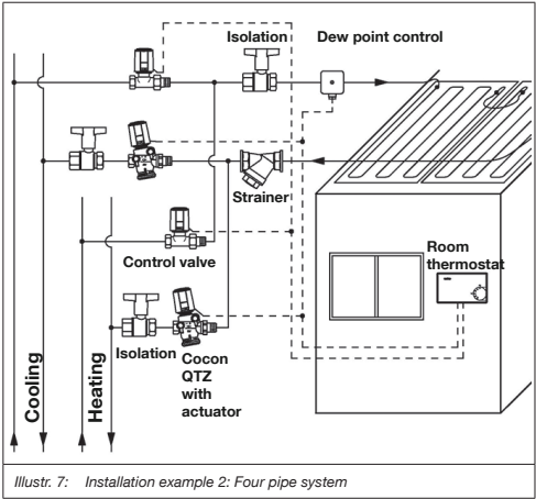
Illust. 7: Installation example 2: Four pipe system
