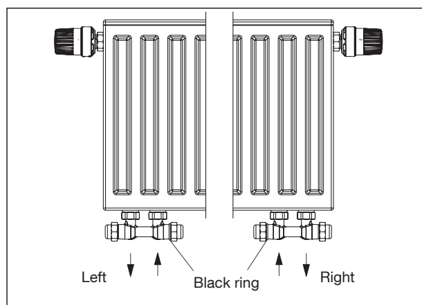
Allocation of the connections of the angle pattern model for left/right hand side connection.
