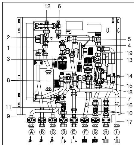
Illustr. 5.1 Construction with high temperature circuit
