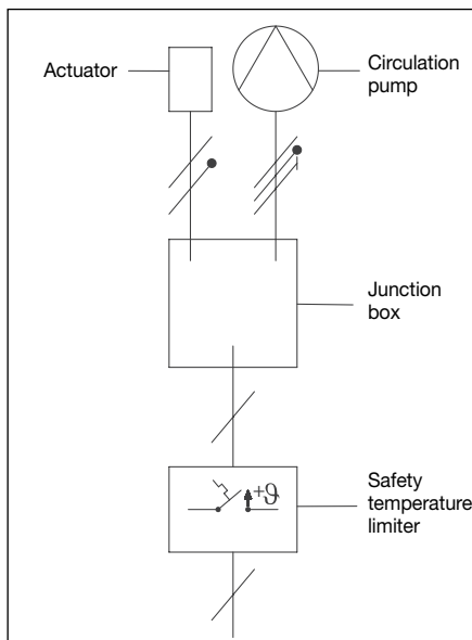
Illustr. 4.1 System illustration cabling
