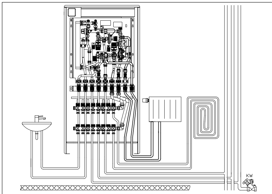
Illustr. 8.5 System illustration
