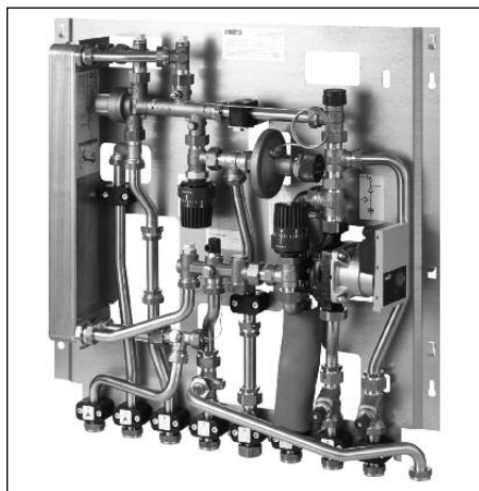
Illustr. 1.1 “Regudis W-HTF” Dwelling station with high temperature circuit
