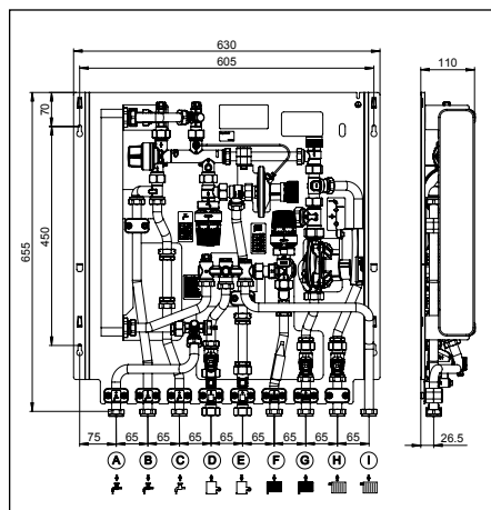
Illustr. 4.2 Dimensions with high temperature circuit
