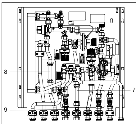
Illustr. 6.3 Installation cold water meter and heat meter
