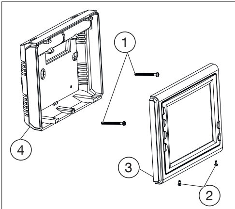
Fig. 4: Montage mural
