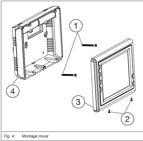
Fig. 4: Montage mural
