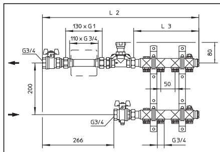
Illustr. 2: Example: Heat meter connection set no. 1, straight pattern, and stainless steel distributor/collector "Multidis SH" for radiator connection, lengths and depth
