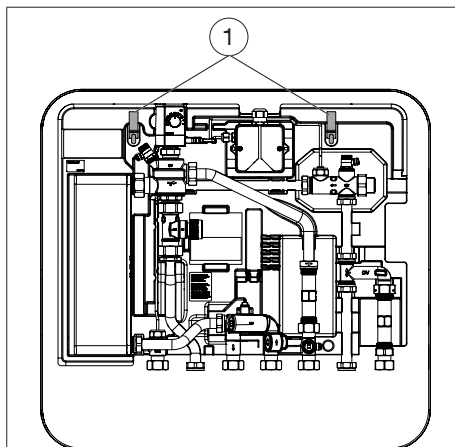
Abb. 3: Position Winkelblech
