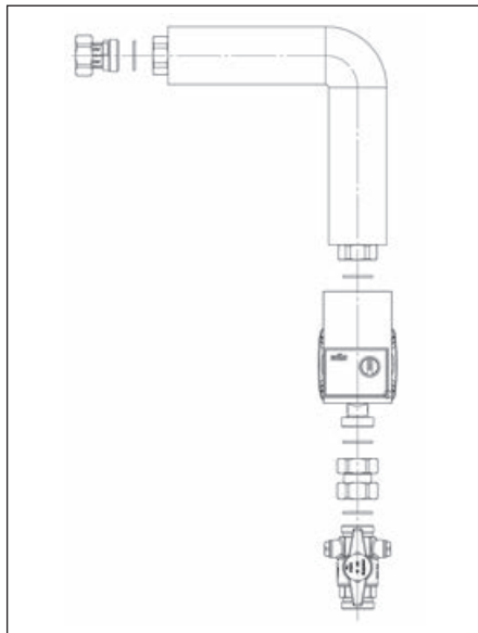
Illustr. 1.4 Circulation connection set with pump Wilo-Yonos PARA Z 15/70 RKC and adapter
