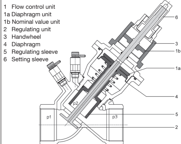
Pressure independent control valve “Cocon QTR”
