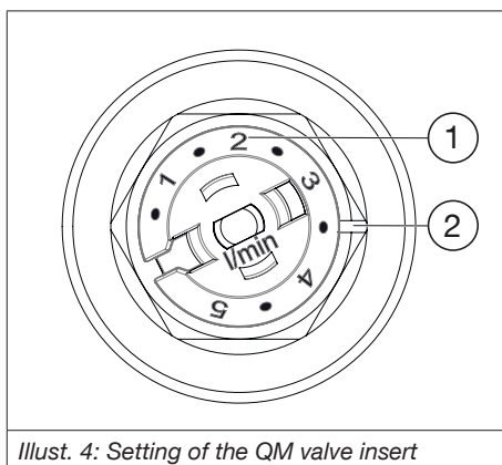
Illust. 4: Setting of the QM valve insert
