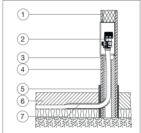
Illustr. 6: Installation cross section
