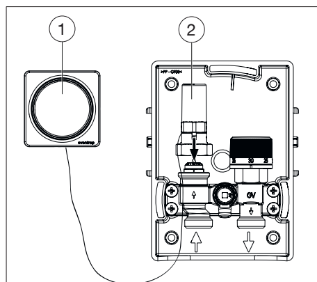
Illustr. 10: Install thermostat with remote control
