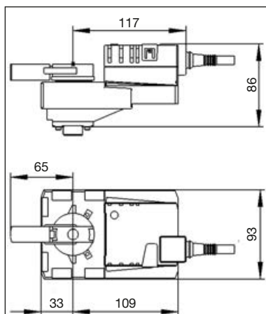
Illustr. 2: Dimensions
