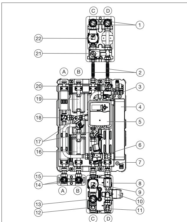
Illust. 2: Construction of the Regudis H-MHT
