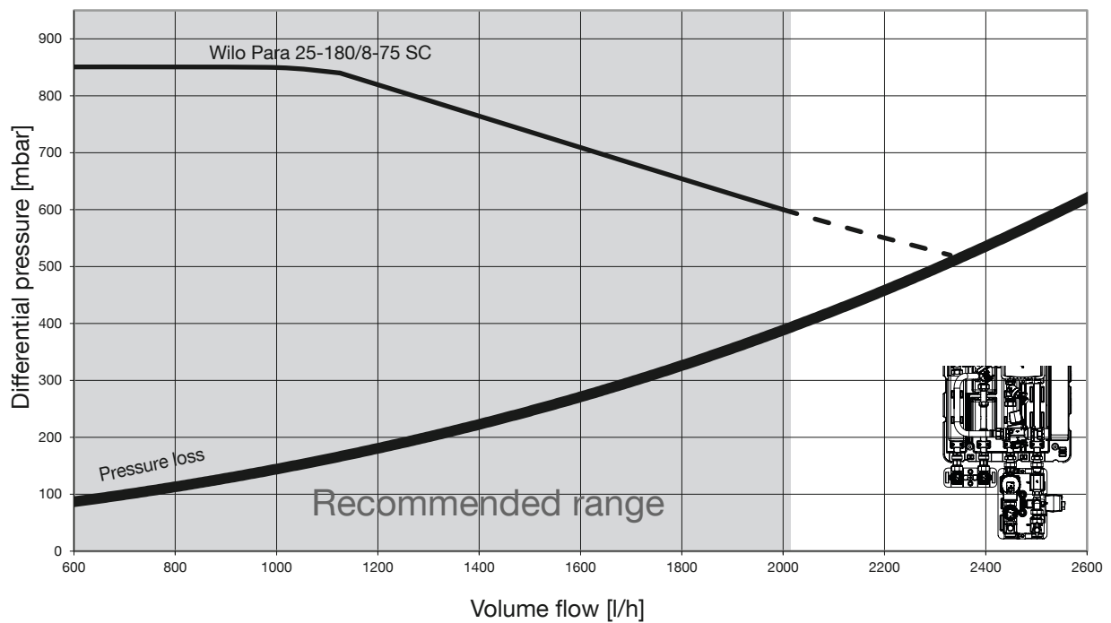
Illust. 6: Pressure loss secondary circuit Regudis H-MHT (HT switching module)
