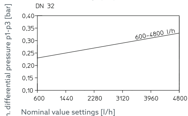
Fig. 13: Minimum differential pressures
