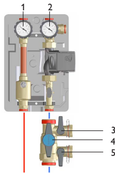
Example: Pump station with filling and flushing unit
