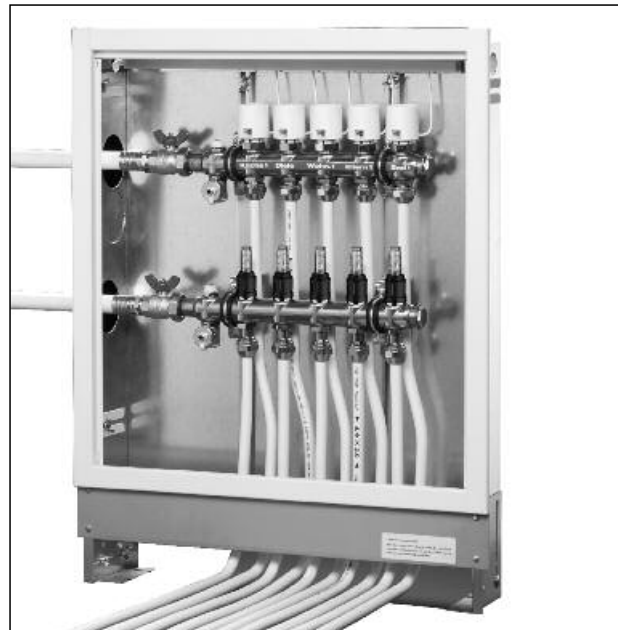
“Multidis SF” Stainless steel distributor/collector Item no. 14041.. and 14042..
