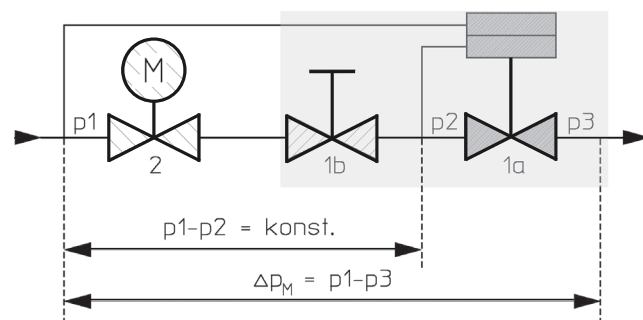
Fig. 3: Operating principle Cocon QTZ, PN 25
