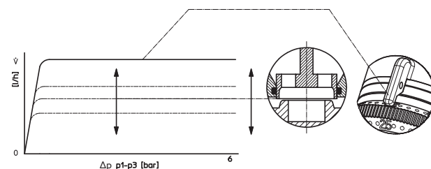
Fig. 4: Differential pressure p_1 - p_3 (bar)
