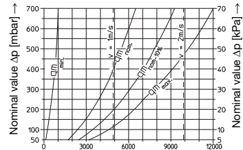
DN 50: kvs = 34.0
