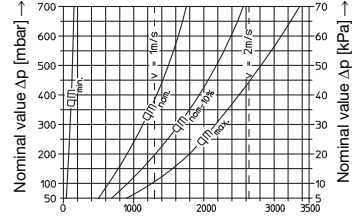
DN 25: kvs = 7.5
