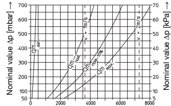
DN 40: kvs = 15.0
