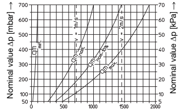
DN 20: kvs = 5.0
