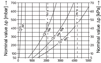
DN 32: kvs = 10.0
