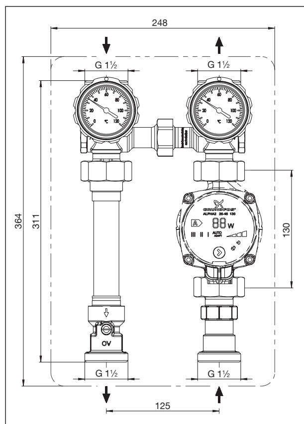
Encombrements Regumat S-130 DN 25
