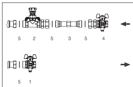
Illustr. 6.2: Heat meter connection set no. 1, straight pattern, extent of supply and location of components for right hand side connection
