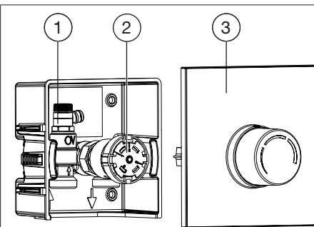
Illustr. 1: Construction “Unibox RTL vario”
