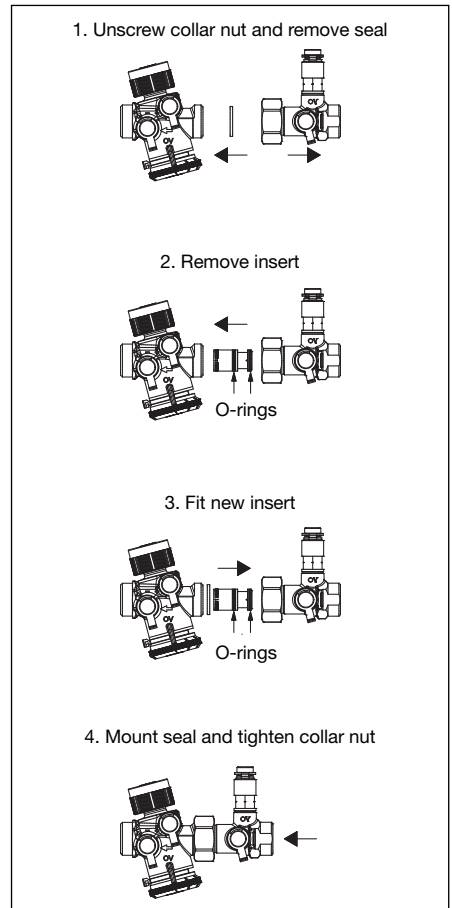
Illustr. 6.3 Replacement of metering station insert
