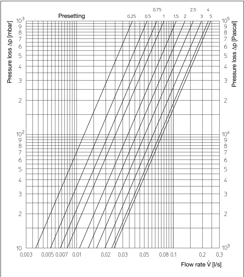
Illustr. 7.3: Chart regulating insert, 2K P-deviation, presetting bypass 2.3 (75%)
