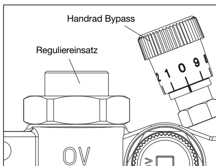
Abb. 6.1 Handrad Bypass
