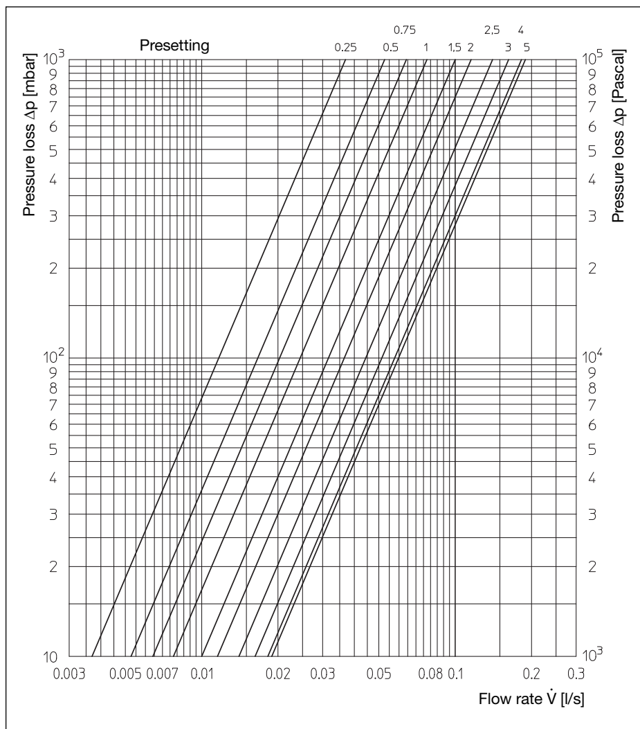
Illustr. 7.1: Chart regulating insert, 2K P-deviation, presetting bypass 1.4 (25%)
