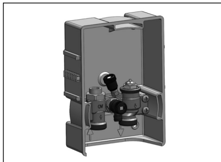
Illustr. 2 “Unibox E BV” item no. 1022676 without cover plate and thermostat for fixing channel with isolating facility (item no. 1022654)
