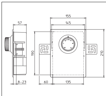
Illustr. 3.1 Dimensions of "Unibox E BV"
