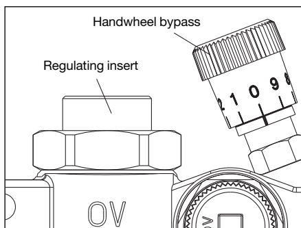
Illustr 6.1 Handwheel bypass
