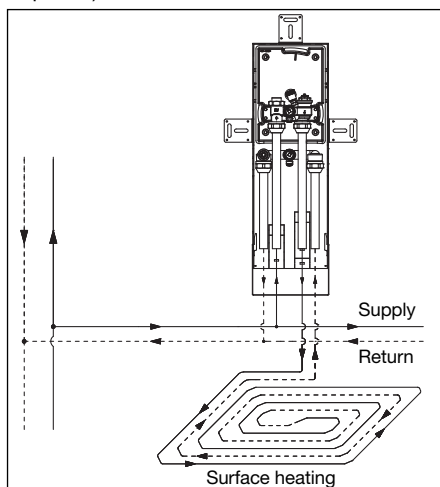
Illustr. 5.5 Installation sketch with "Unibox E BV" in the fixing channel, item no. 1022654
