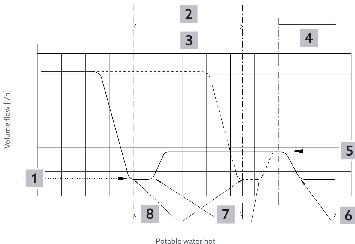
Fig. 6: Thermal control behaviour
