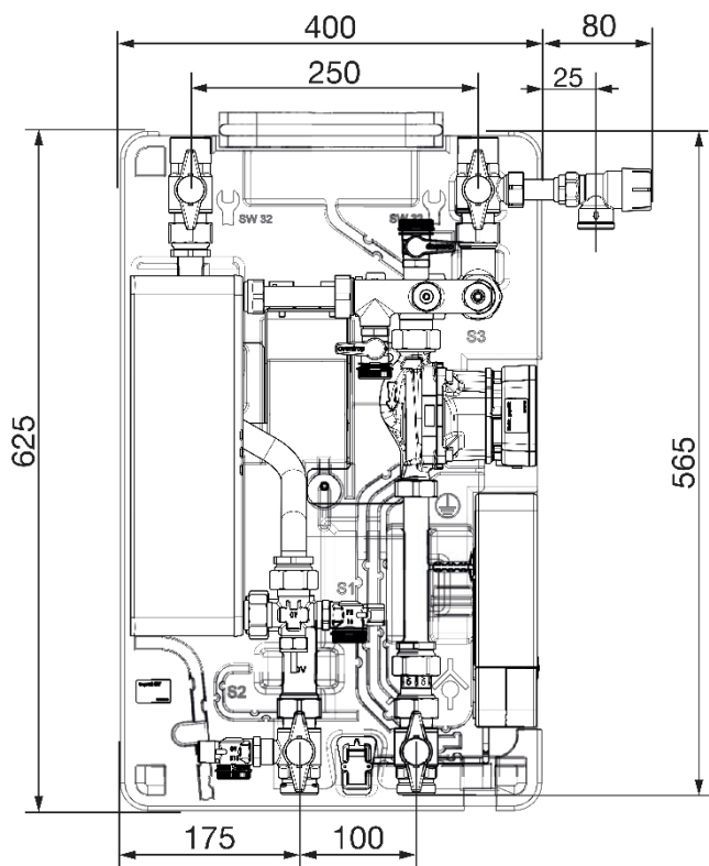
Abmessungen Regumaq X-45 (Front)
