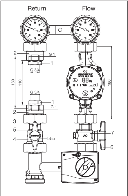
Illustr. 5.2 Heat meter installation set for "Regumat M3-180" DN 25 with pump ball valve (2015)
