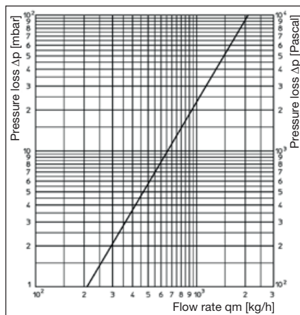
Chart 1: Pressure loss heat meter connection set no. 1
