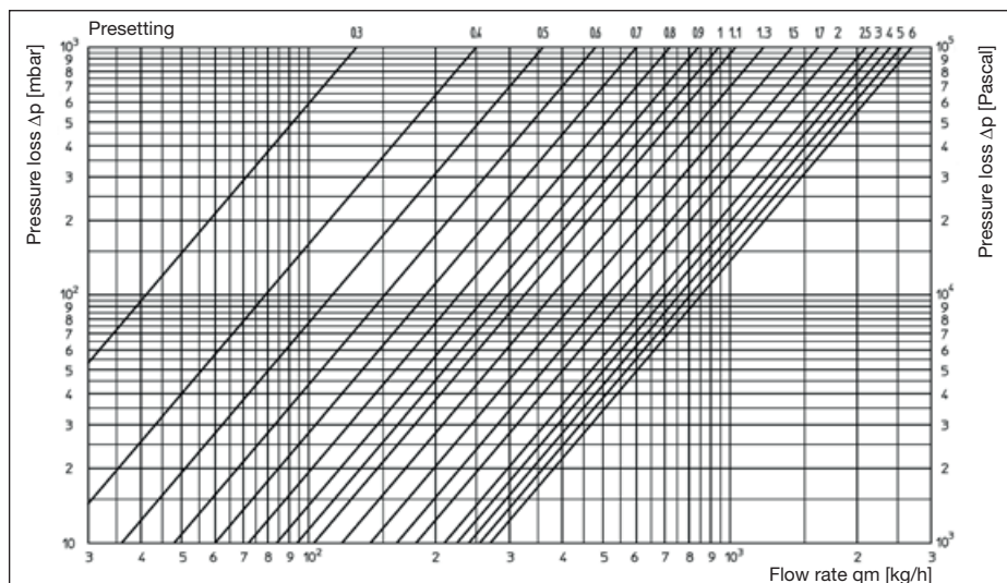
Chart 2: Pressure loss double regulating and commissioning valve "Hycocn VTZ" DN 20
