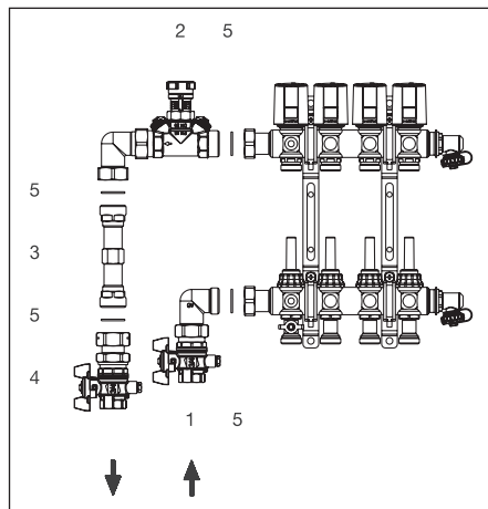
Illustr. 6.1: Heat meter connection set no. 1, angle pattern, extent of supply and location of components for left hand side connection
