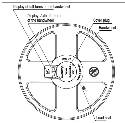
Illustr. 7 Locking the handwheel DN 200 - DN 300
