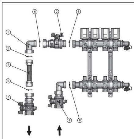
Illustr. 4: Heat meter connection set, angle pattern, extent of supply and location of components for left hand side connection.
