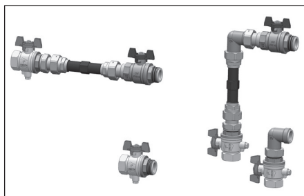
Illustr. 1 Heat meter connection set, straight and angle pattern
