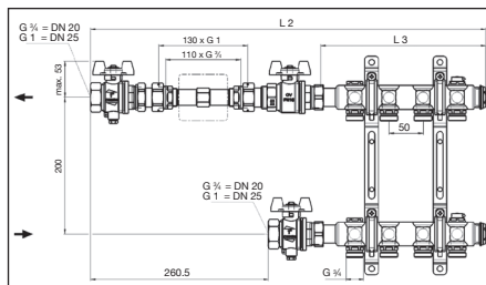
Illustr. 3 Heat meter connection set, straight pattern and stainless steel distributor "Multidis SH" for radiator connection, lengths
