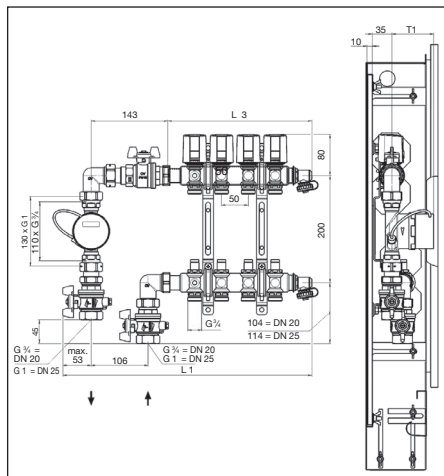
Illustr. 2 Example: Heat meter connection set, angle pattern and stainless steel distributor/collector "Multidis SFQ" for surface heating and cooling systems, lengths and depths
