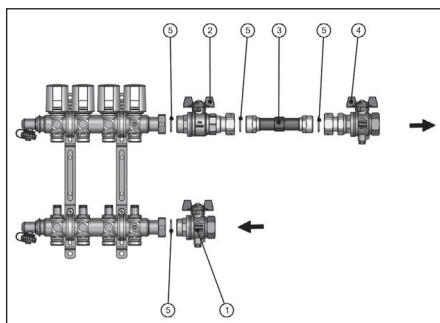
Illustr. 5: Heat meter connection set, straight pattern, extent of supply and location of components for right hand side connection
