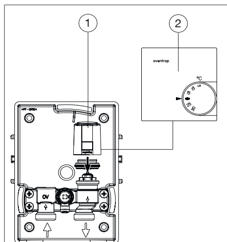
Illust. 9: Installation of the room thermostat with actuator
