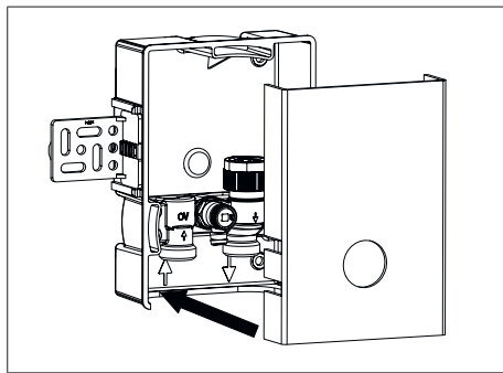
Illust. 7: Fitting of the protection cover
