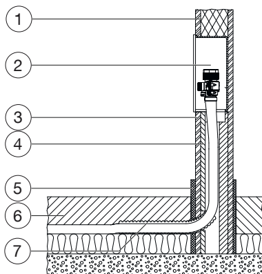
Illust. 4: Installation cross section
