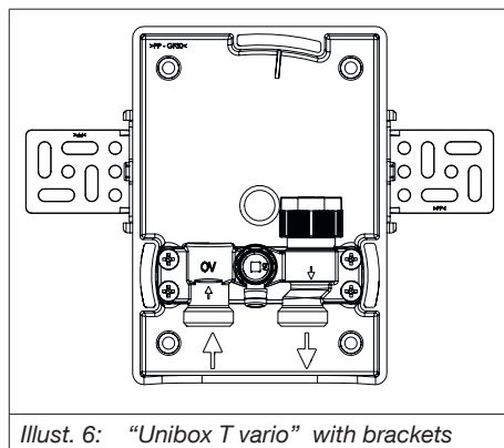
Illust. 6: “Unibox T vario” with brackets
