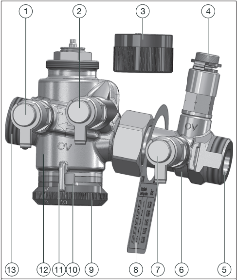
Abb. 1: “Cocon QTZ” with metering orifice
