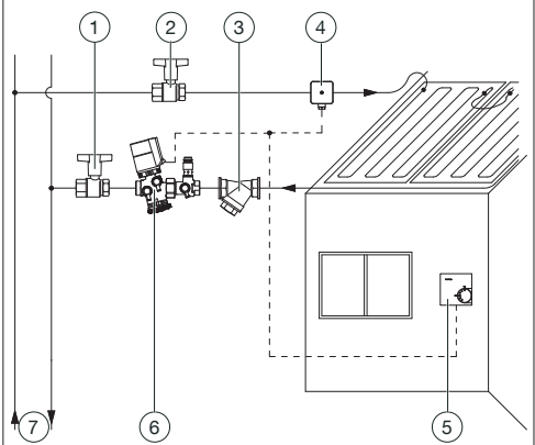
Abb. 6: Installation example 1: Dual-line system
