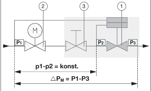
Abb. 3: “Cocon QTZ” functional diagram
