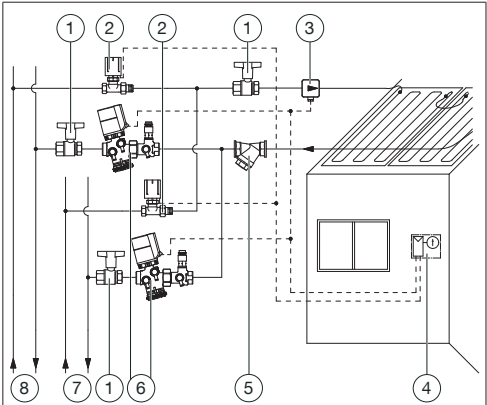
Abb. 7: Installation example 2: Four-line system
