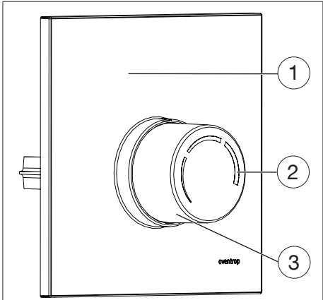
Illust. 4: Handwheel
