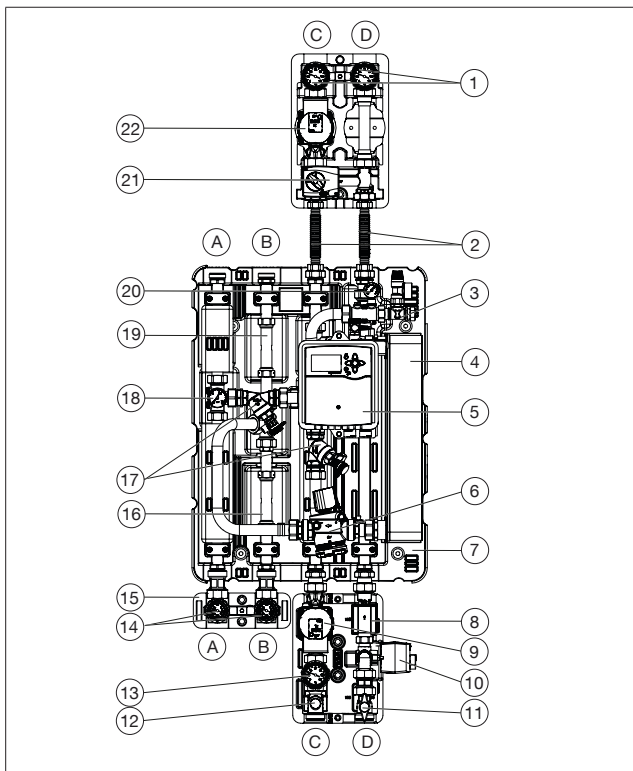
Illust. 2: Construction of the Regudis H-MHT
