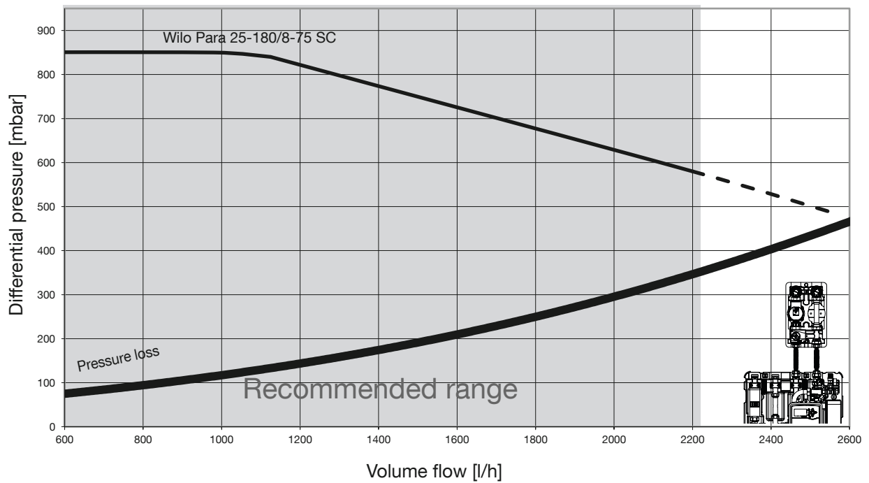
Illust. 5: Pressure loss secondary circuit Regudis H-MHT (Regumat M 3)
