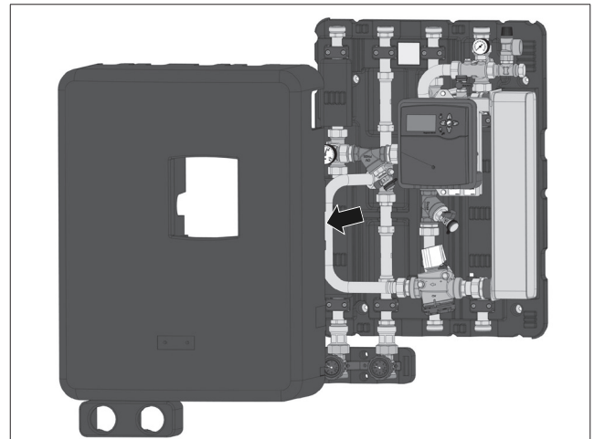
Illust. 26: Removal of the front insulation shells
