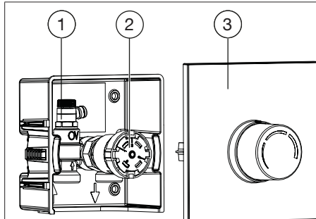
Illustr. 1: Construction “Unibox RTL vario”
