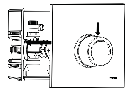
Illustr. 6: Fitting of the cover with handwheel
