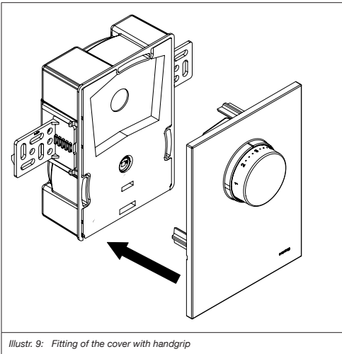
Illustr. 9: Fitting of the cover with handgrip
