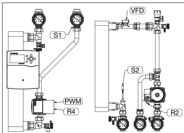
Illustr. 3: "Regumaq XZ-30-B" Primary and secondary circuit
