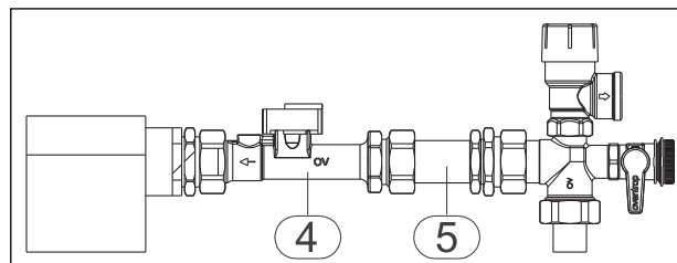
Illustr. 2: Installation Vortex flow sensor
