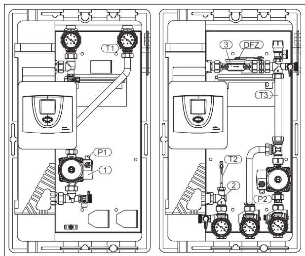
Illustr. 1: "Regumaq XZ-30" Primary and secondary circuit
