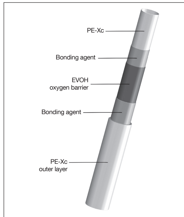
“Copex” PE-Xc plastic pipe (Dimension 20 x 2,5 mm, 26 x 3 mm, 32 x 3 mm)
