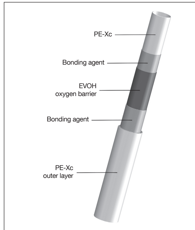
“Copex” PE-Xc plastic pipe (dimension 14 x 2 mm, 16 x 2 mm, 17 x 2 mm, 20 x 2 mm)
