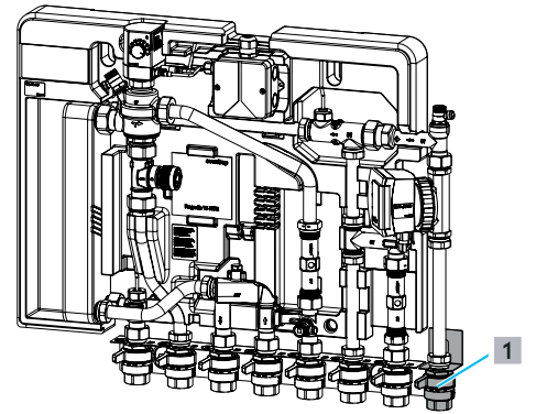
Fig. 1: Installation location
