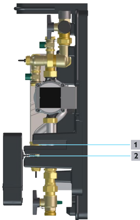
Abb. 28: Montageposition
