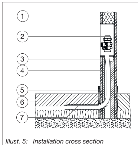
Illust. 5: Installation cross section
