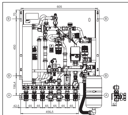
Illustr. 6.1 Connection scheme ball valve connector block
